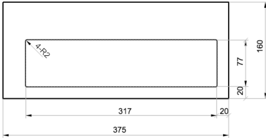
Top board
